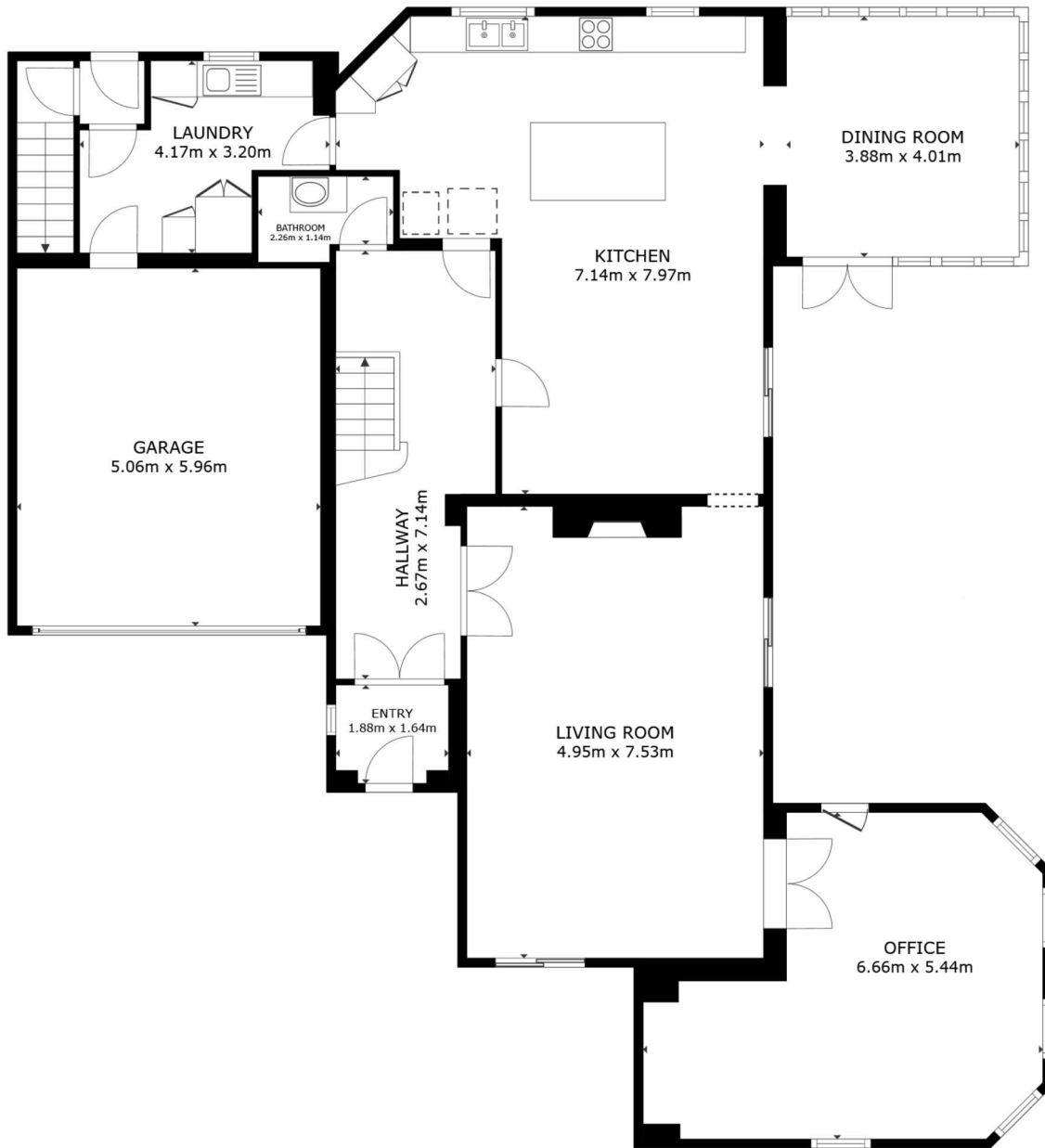
FLOOR 1
